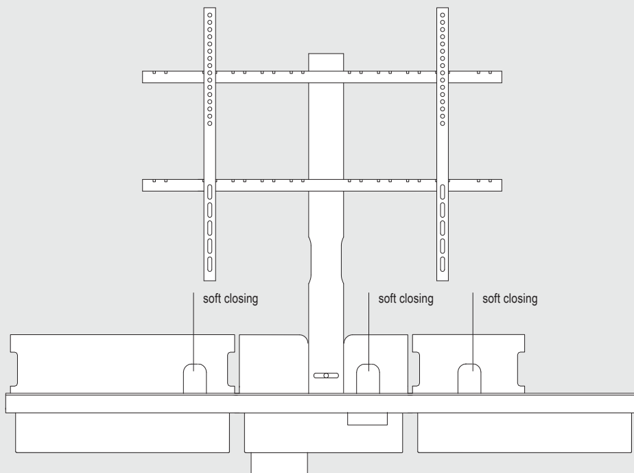
fronte / front
