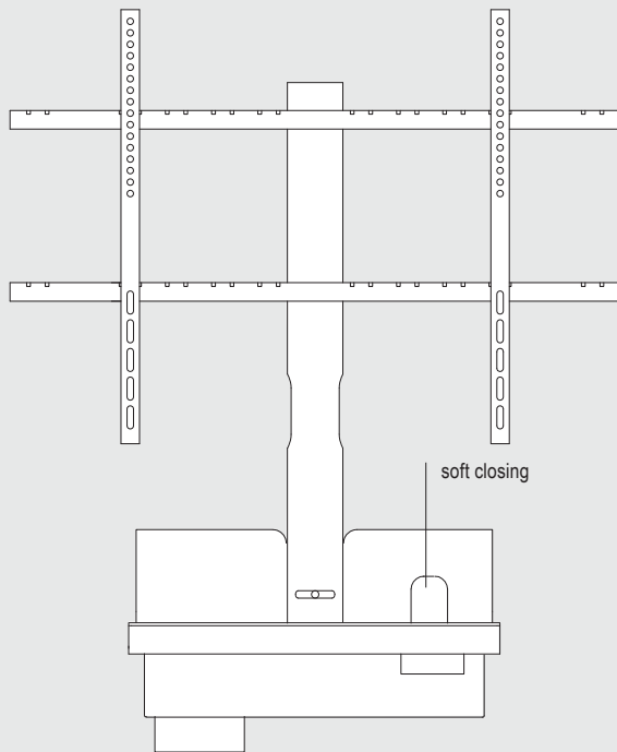
fronte / front
