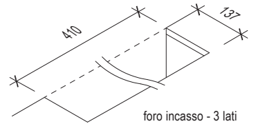
foro incasso - 3 lati recessed hole - 3 sides
